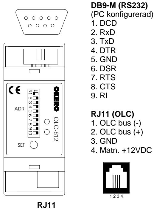
Figur 1. OLC812 frontvy
