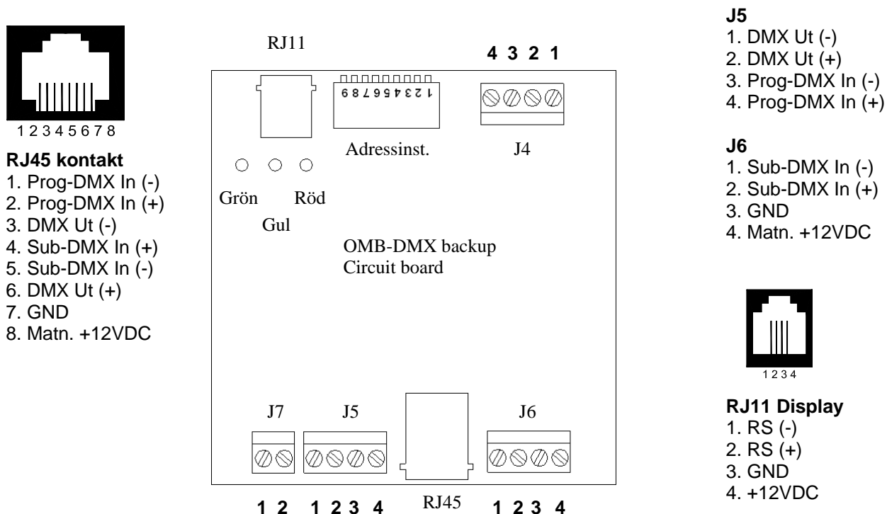
Figur 1. OLC306 toppvy
